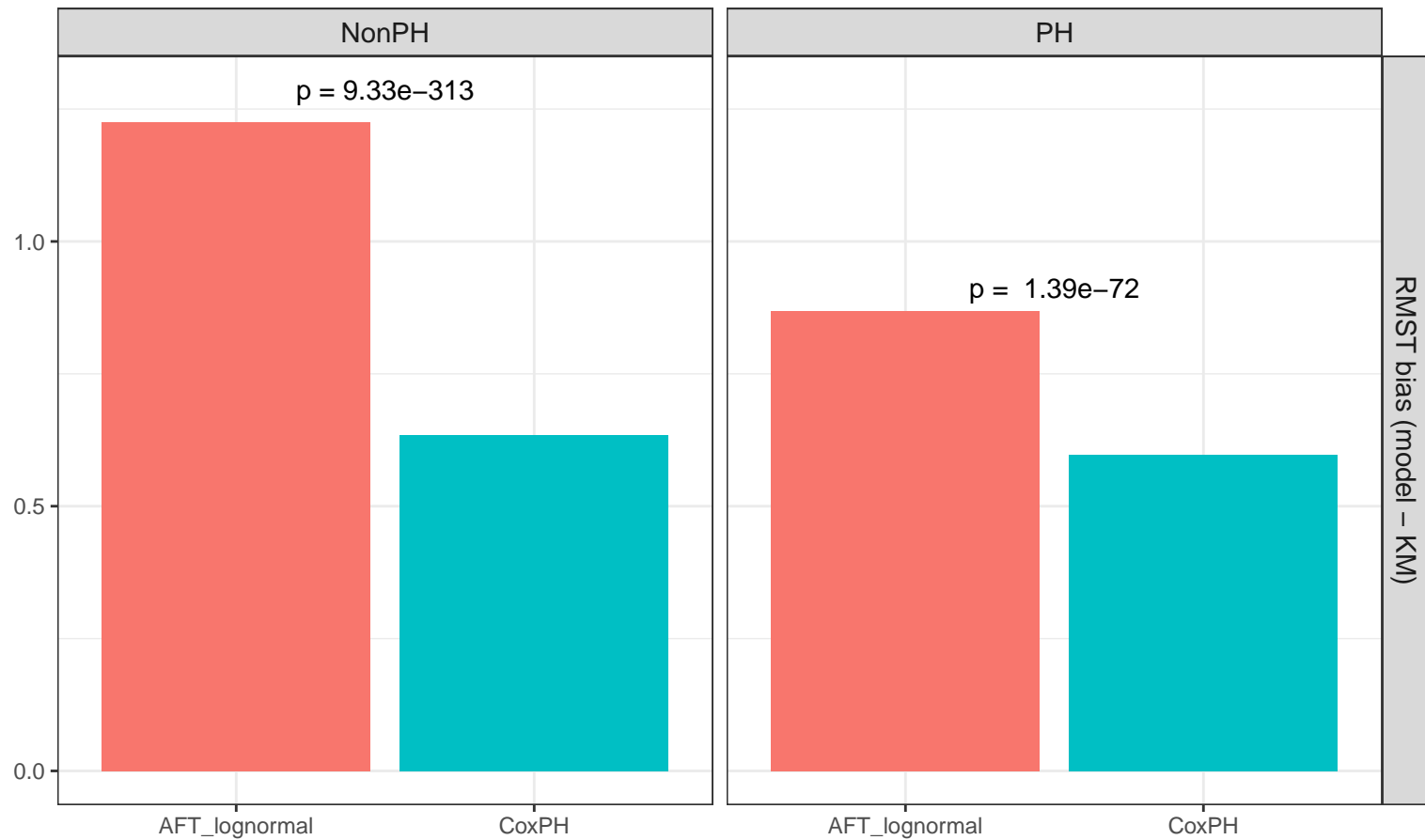
RMST bias under PH vs Non-PH scenarios
