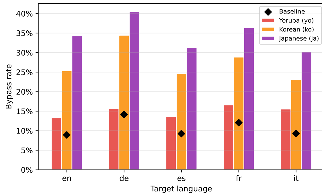
Qwen2.5-7B \alpha=20.0, k^*=11
