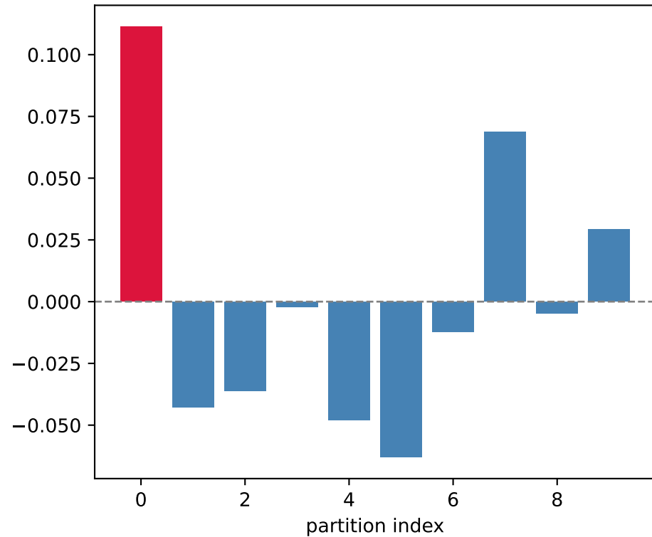
Qwen2.5-7B-Instruct
