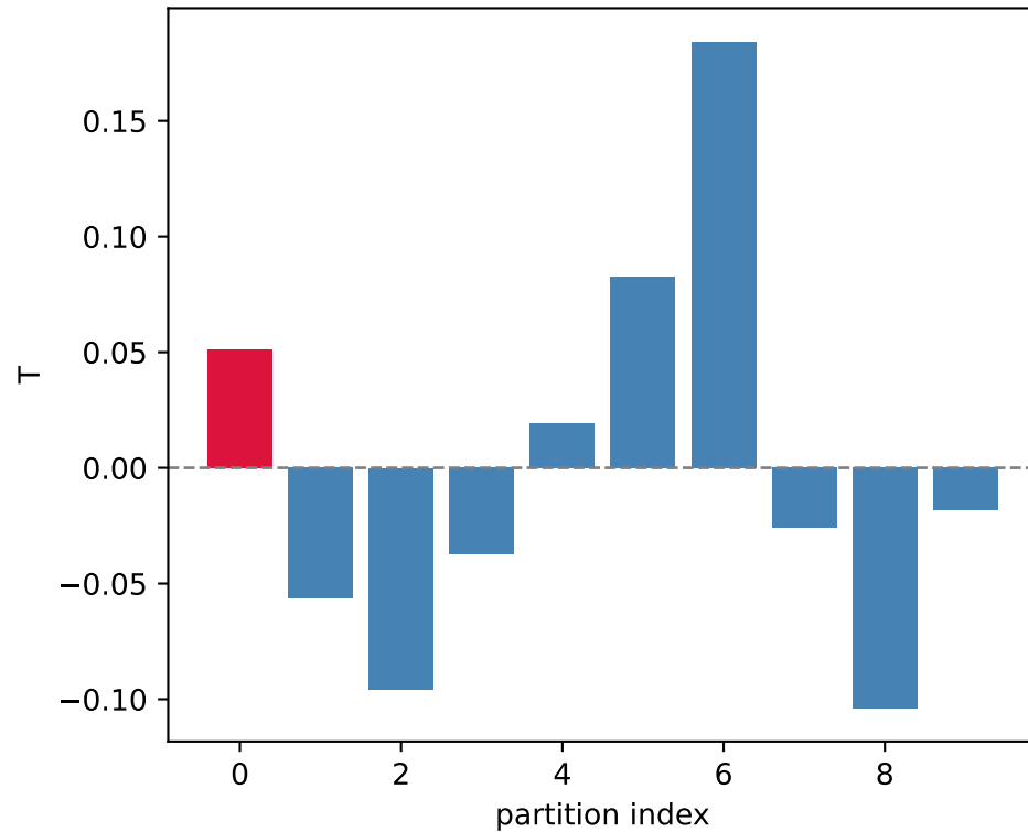
Meta-Llama-3.1-8B-Instruct
