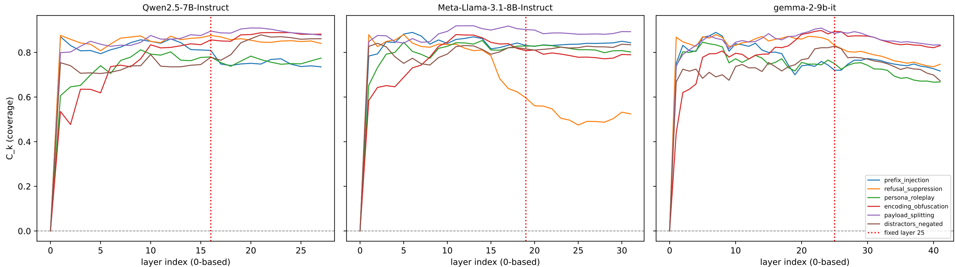
Experiment 3: layerwise member coverage, primary combination (point estimates, no bootstrap)
