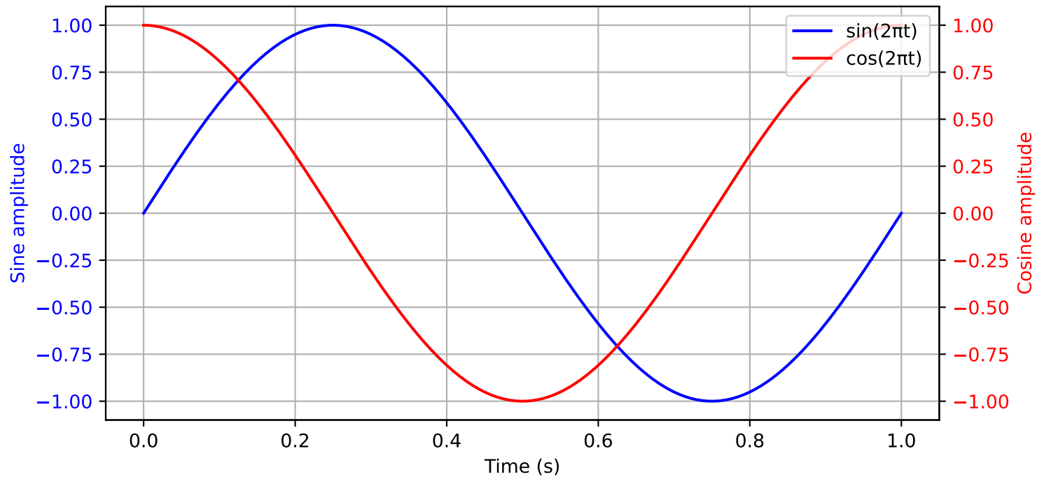
Sine and Cosine
