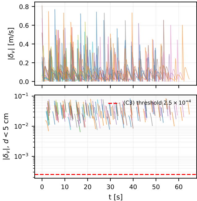
inner-loop velocity error, 12 runs
