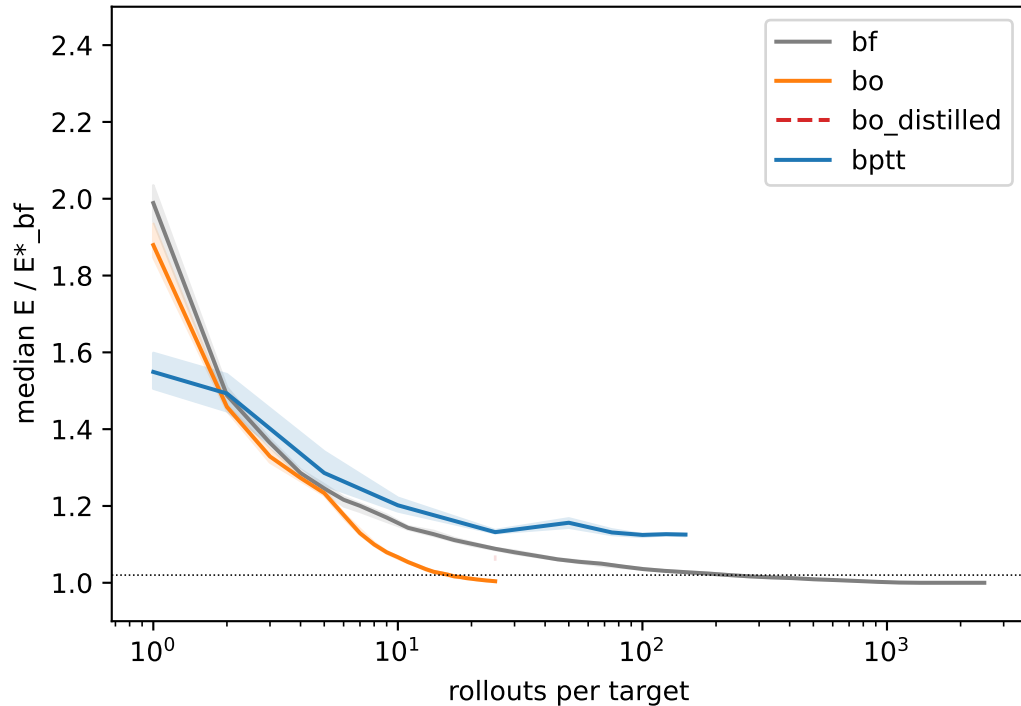
H1: sample efficiency (10 seeds, IQR band)
