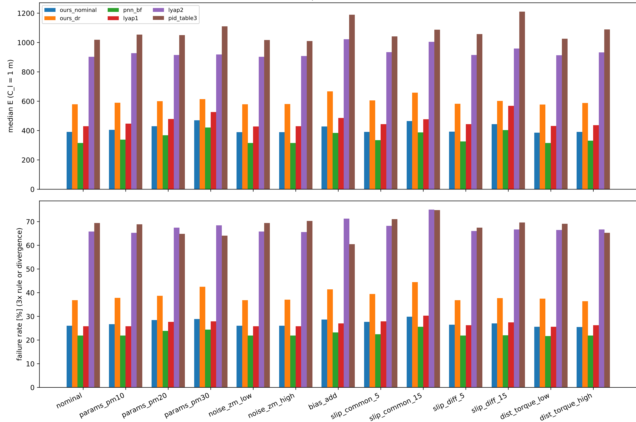
H3: robustness across labeled perturbation conditions (500 MC runs each)
