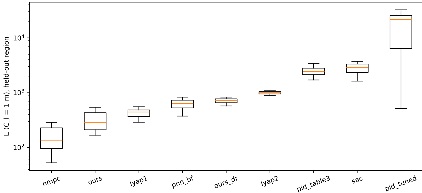
Generalization: held-out workspace d \in [1.0, 1.5] , |\theta| \in [0.7\pi, 0.9\pi]
