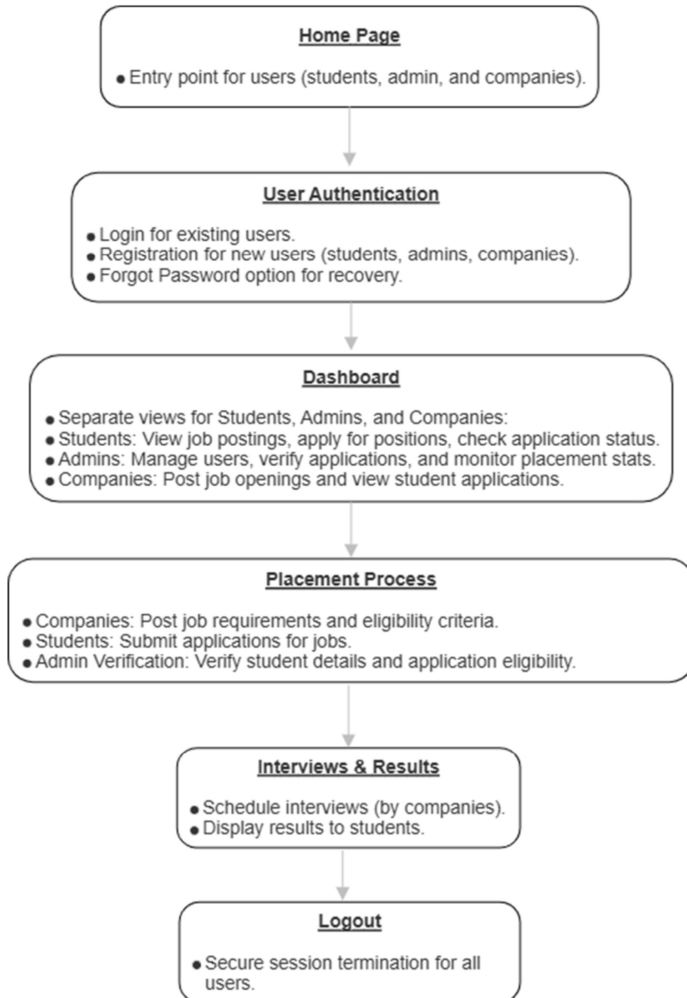
Fig: WORKING PROCESS OF PLACEMENT CELL WEB APP
