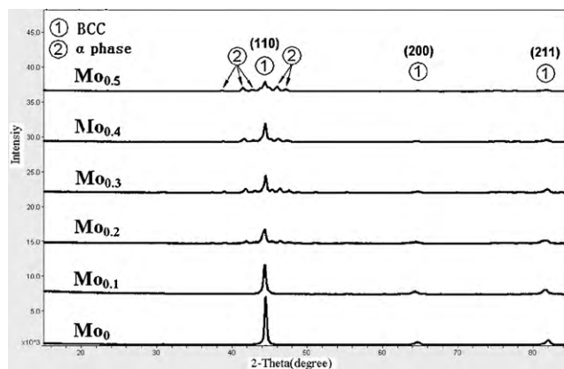
Fig. 1. XRD patterns of as-cast AlCoCrFeNiMo x ( x = 0, 0.1, 0.2, 0.3, 0.4 and 0.5 ) alloys.
