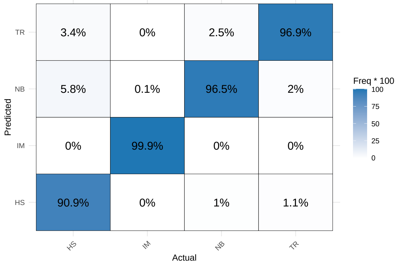
Confusion Matrix: k-NN
