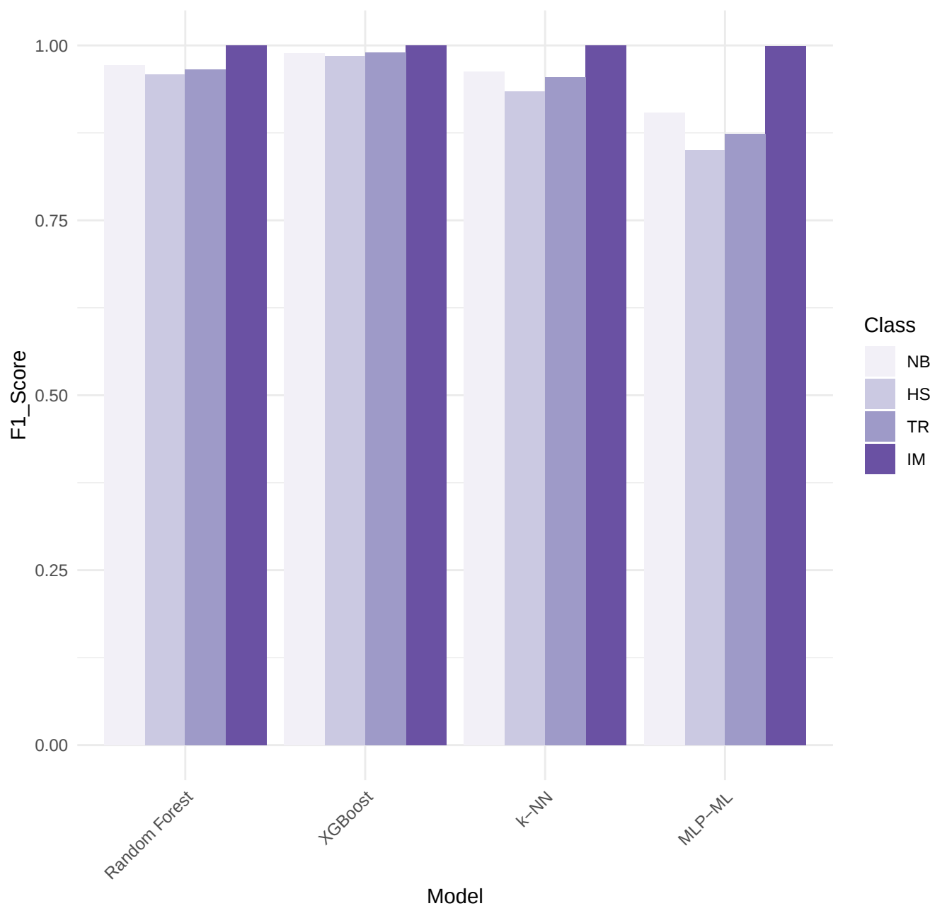
F1 Score per Model and Class
