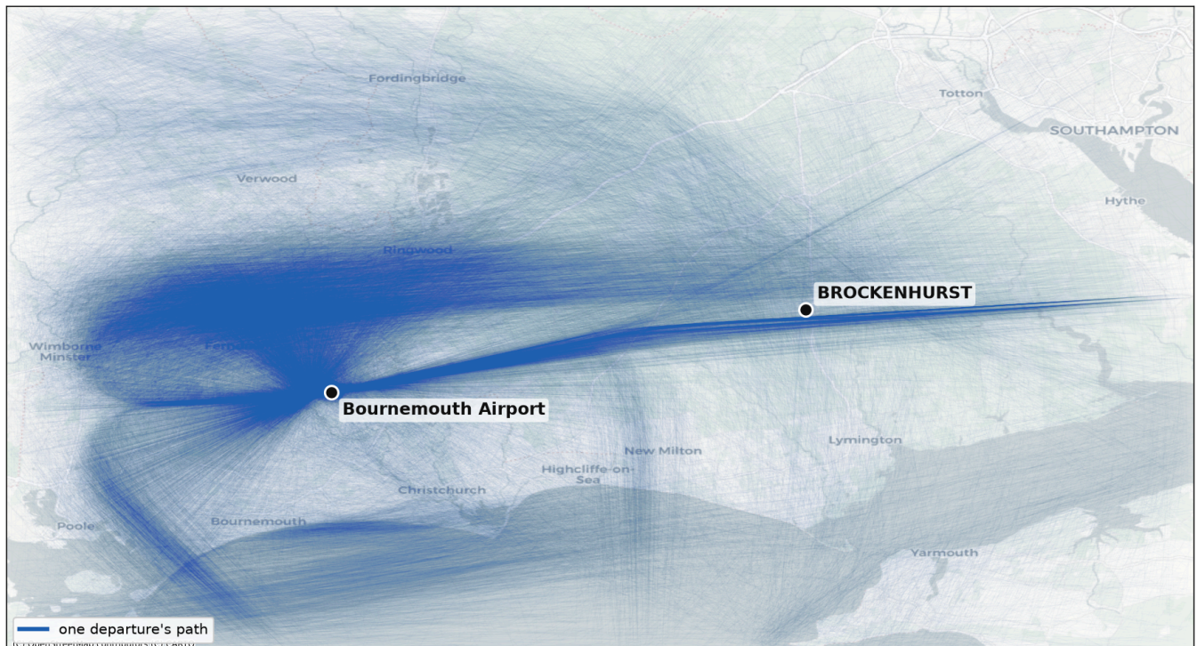
Every Bournemouth departure fans out over Brockenhurst on easterly ops 2023 to 2025 (22,320 departures) - their own GPS tracks
