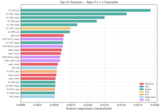
Fig. 4. AD feature importance, tuned Ensemble on F_{++} (notebook 03). Oil-pressure statistics dominate; colors denote sensor groups.
