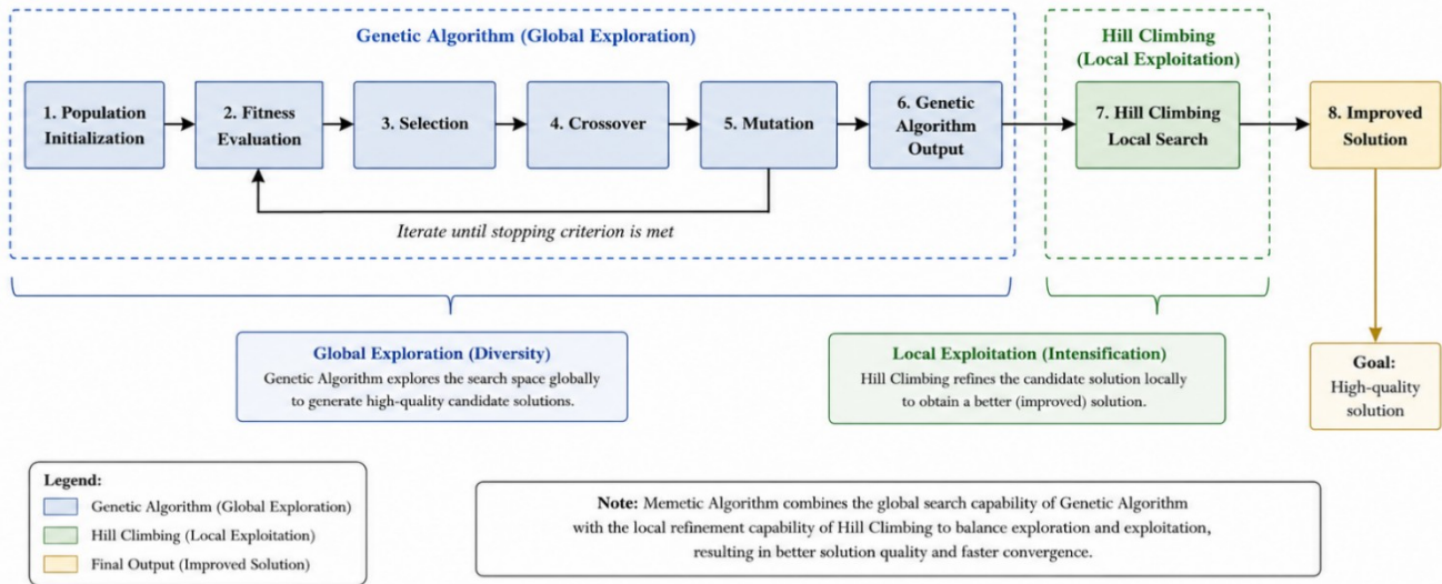
Gambar 2. 3 Genetic Algorithm dan Hill Climbing
