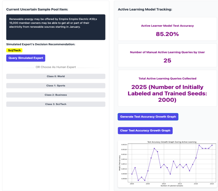
Figure 9: Active Learning Interface State After Generating Test Accuracy Growth Graph Up to 25 User Queries
