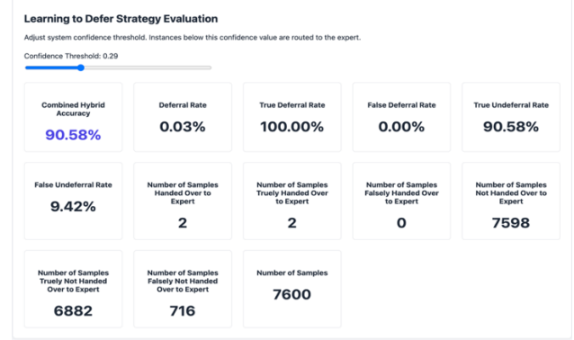
Figure 4: Learning to Defer Strategy Evaluation When Confidence Threshold is 0.29
