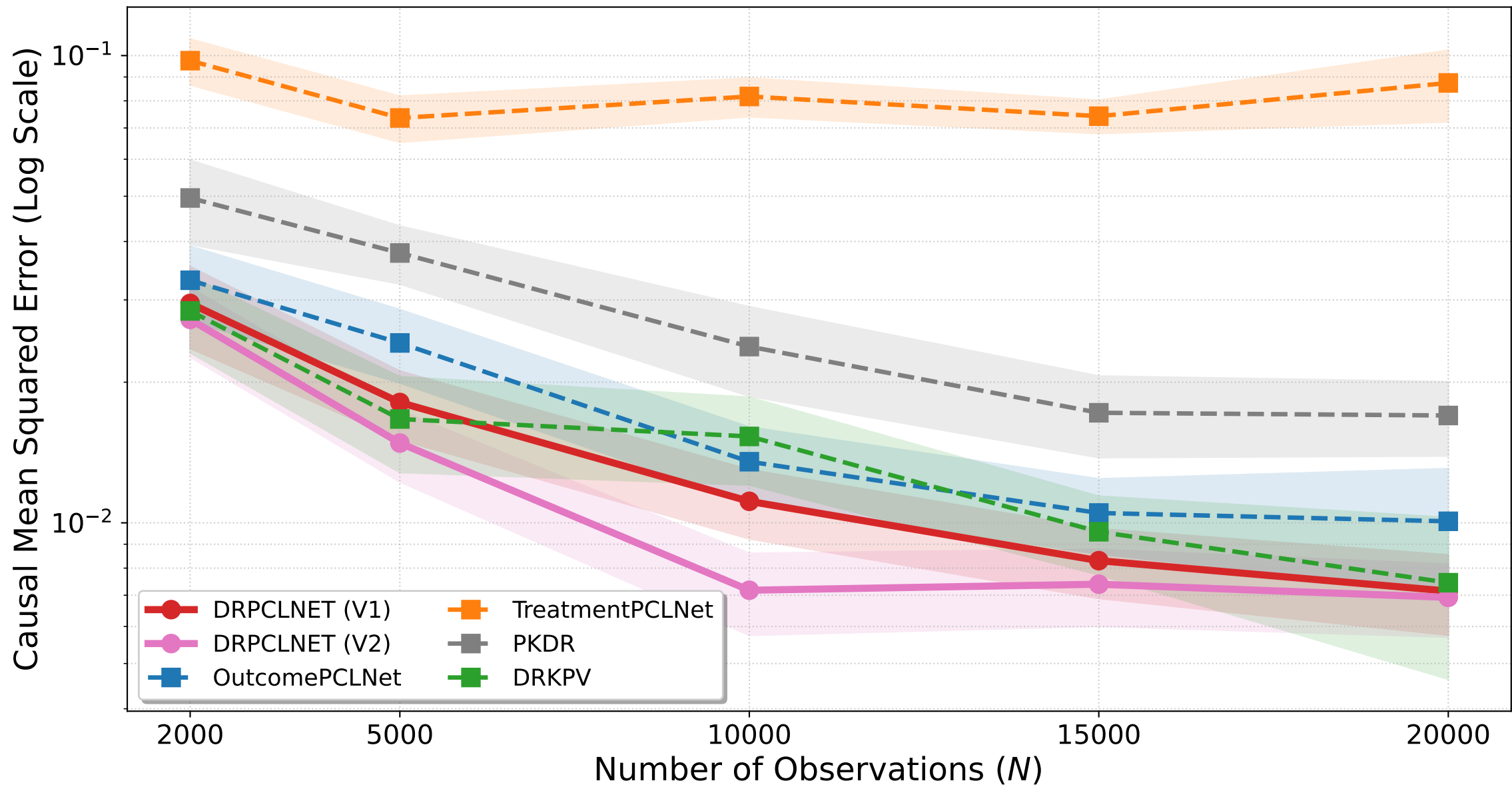
Low Dimensional Dose Response (Mean with 95% CI)
