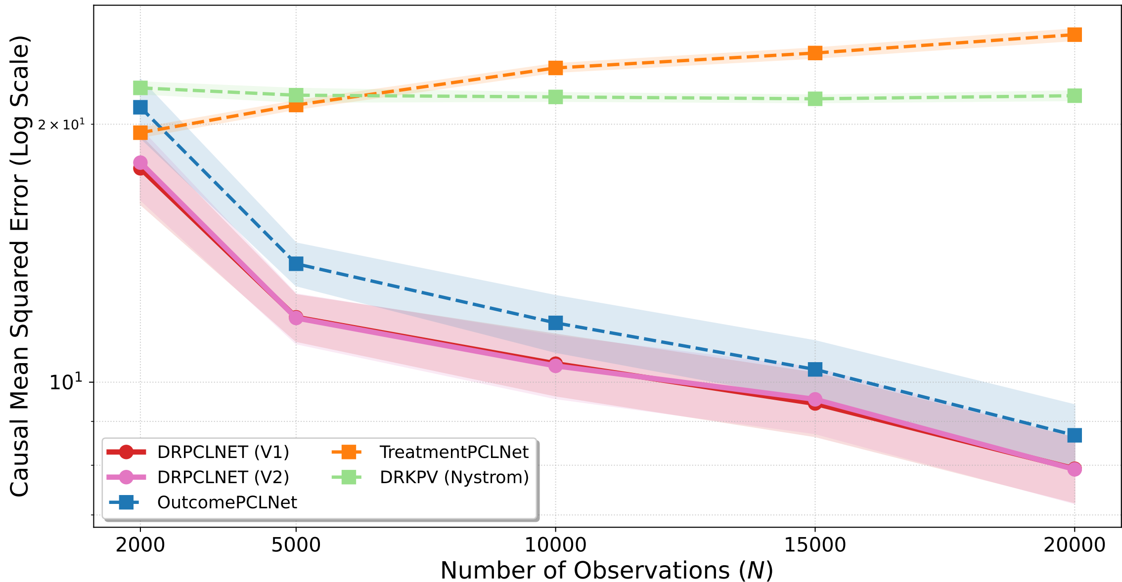
dSprite Dose Response (Mean with 95% CI)
