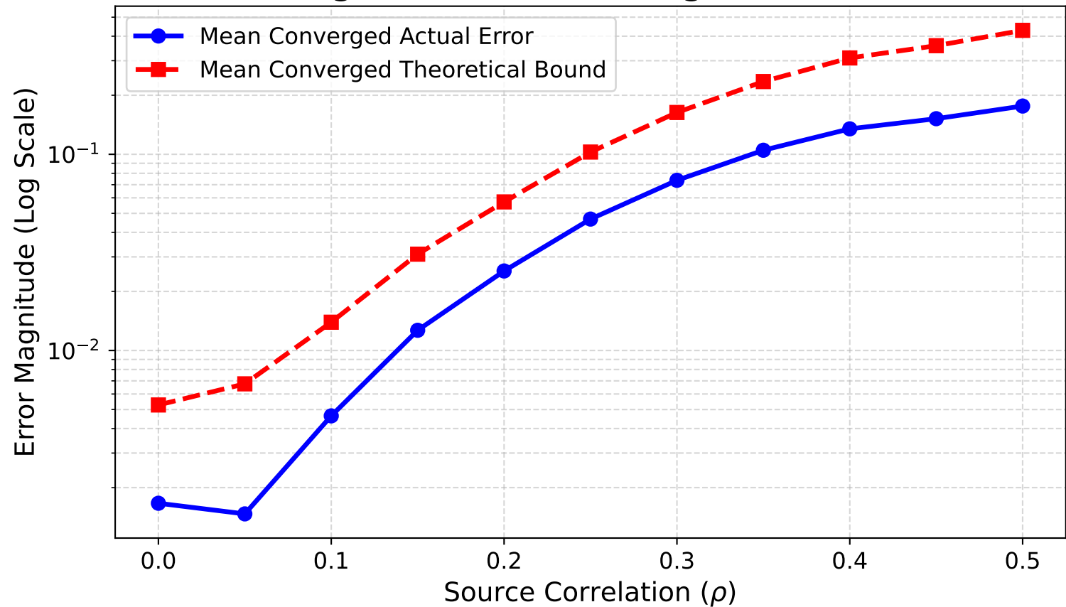
Mean Surrogate Error at Convergence vs. Correlation
