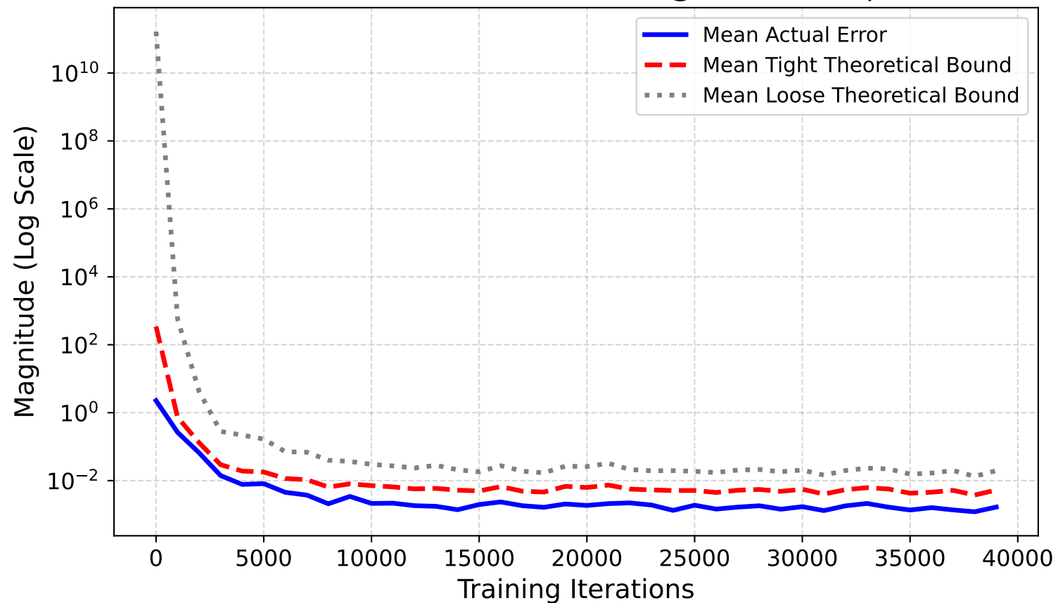
Time-Evolution of Mean Surrogate Error ( \rho = 0.0 )
