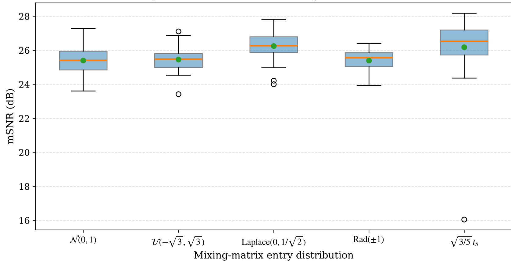
Antisparse ablation: effect of mixing-matrix distribution
