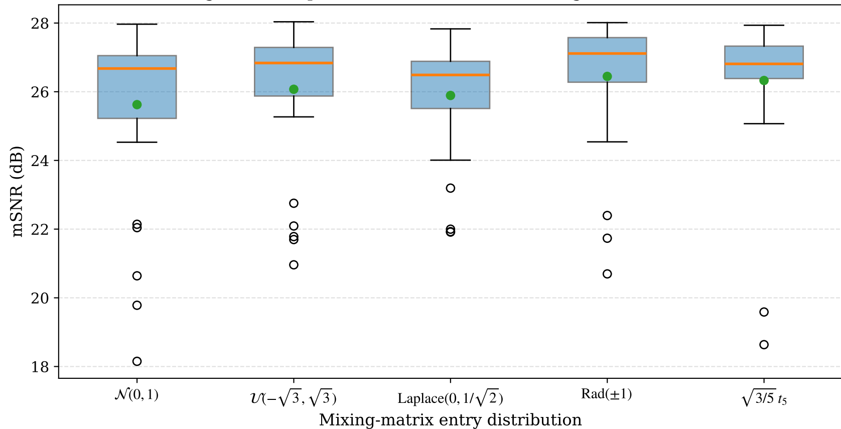
Nonnegative antisparse ablation: effect of mixing-matrix distribution
