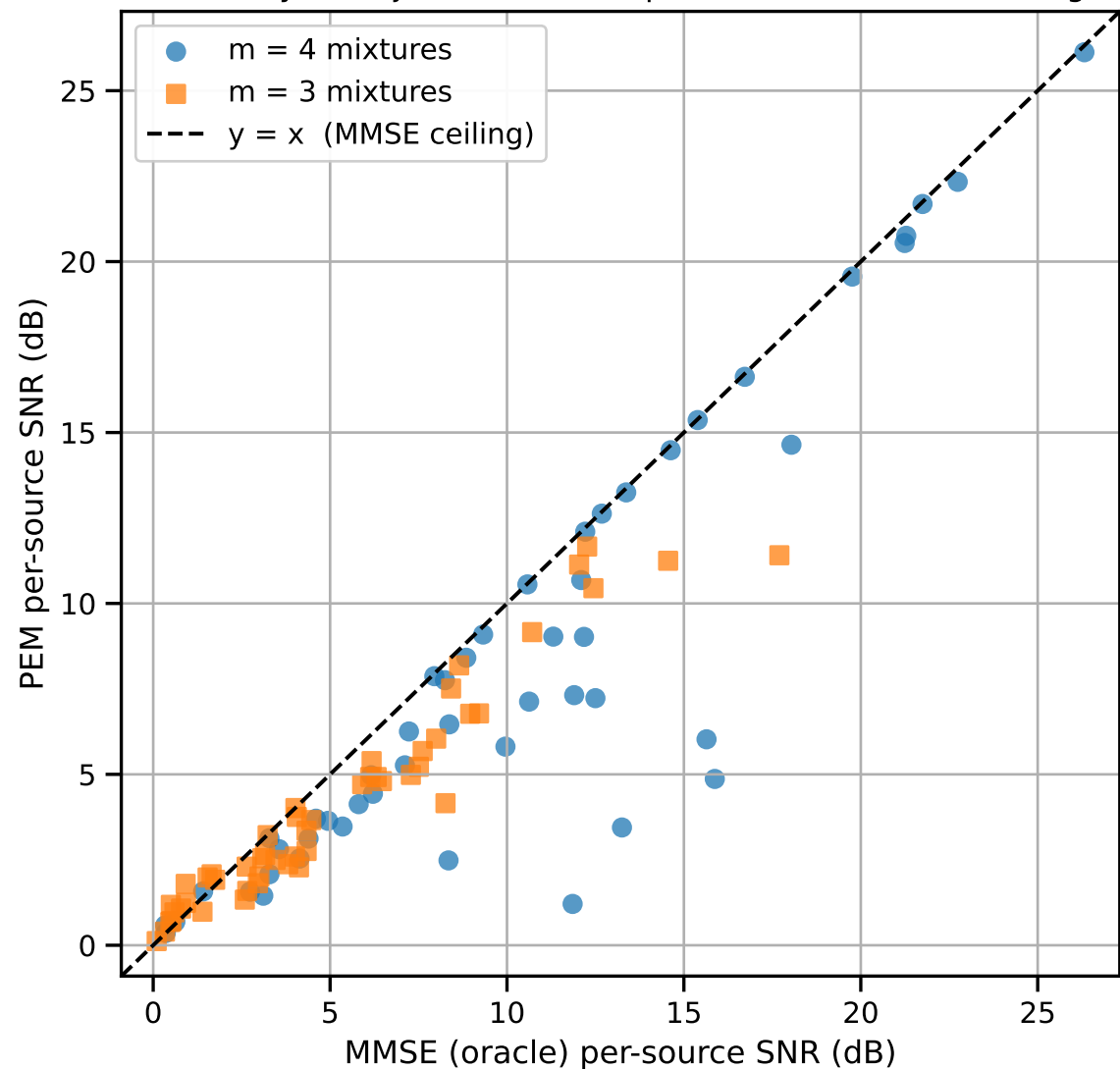
PEM stays on / just below the optimal-linear (MMSE) ceiling
