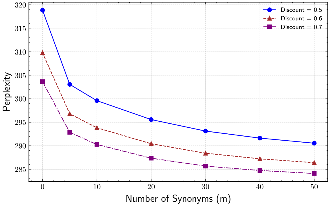
GLOVE - Kneser-Ney
