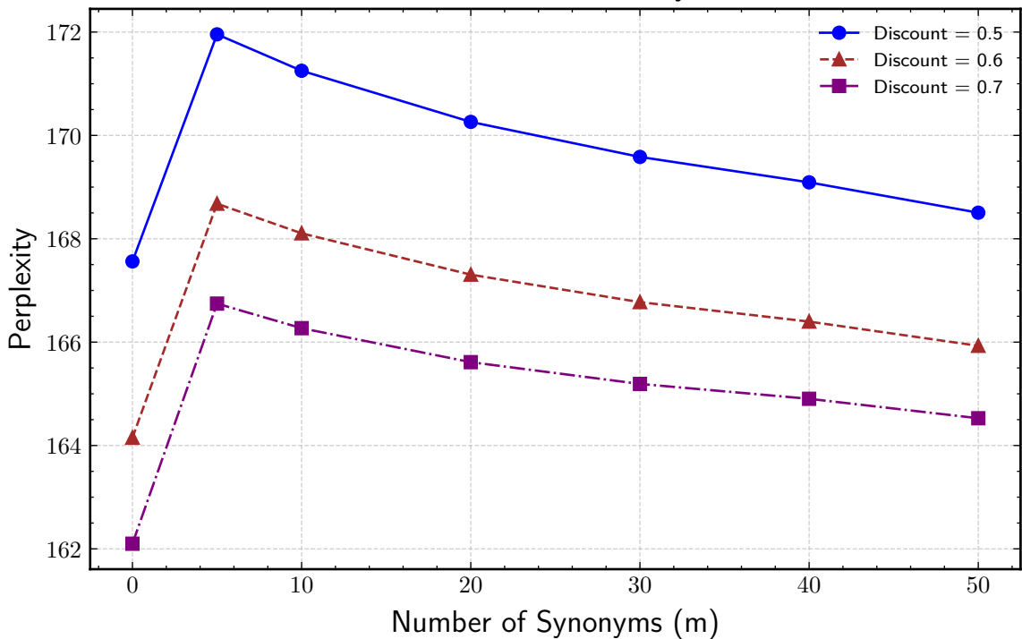
GPT2 - Kneser-Ney
