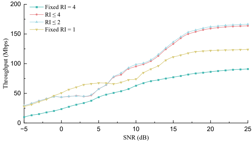
Figure 6: Downlink throughput performance under adaptive and fixed-rank configurations
