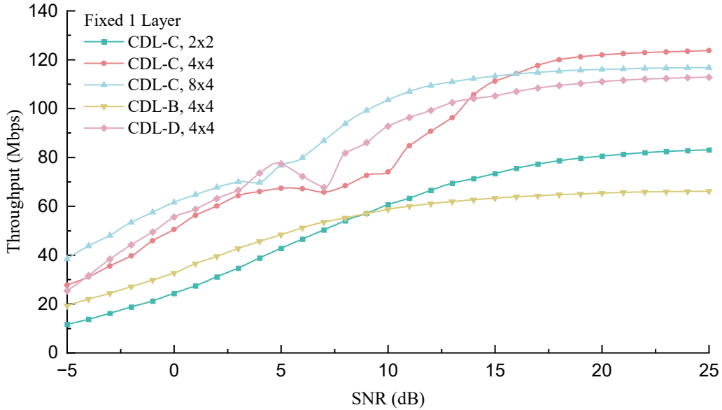
Figure 9: Downlink throughput comparison under fixed one-layer transmission
