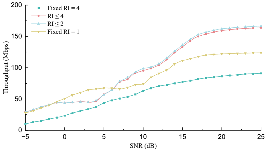
Figure 6: Downlink throughput performance under adaptive and fixed-rank configurations
