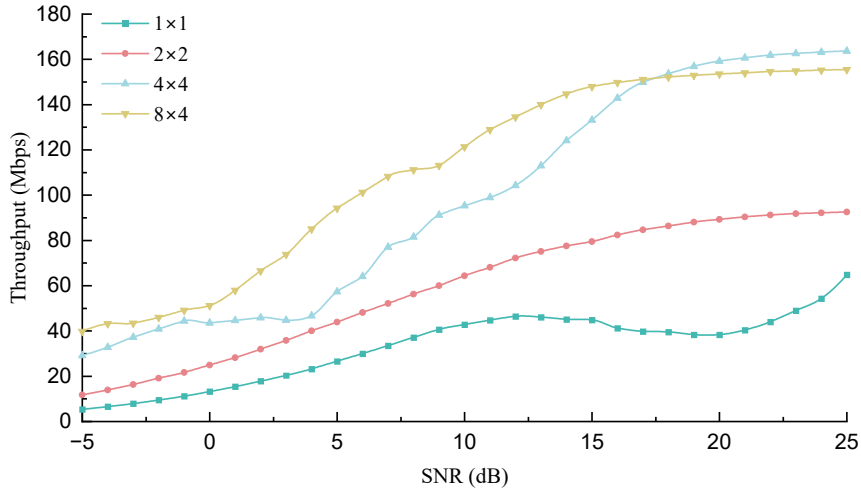
Figure 7: Downlink throughput performance under different MIMO configurations
