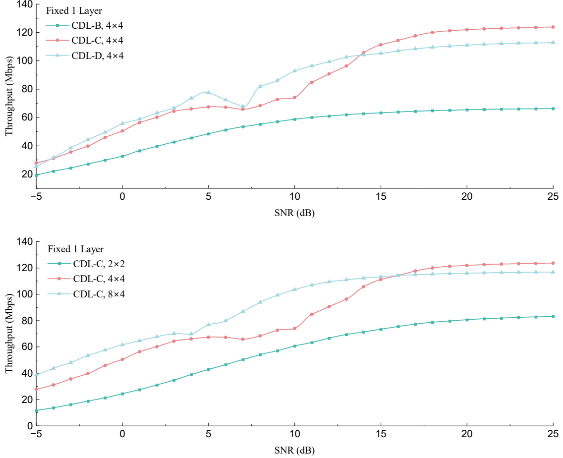
Figure 9: Fixed one-layer downlink throughput comparison across CDL channel profiles and MIMO configurations
