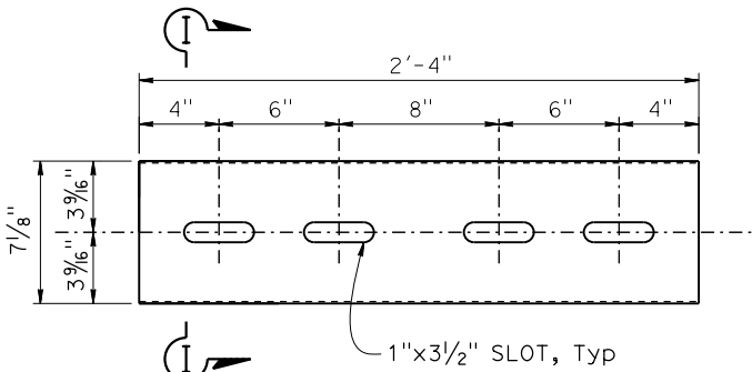
STANDARD SLEEVE DETAIL (FOR HSS8x3x5/16 RAIL)
