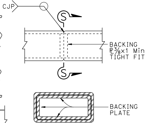
SECTION S-S
