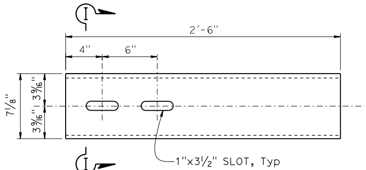
EXPANSION SLEEVE DETAIL (FOR HSS8x3x5/16 RAIL)
