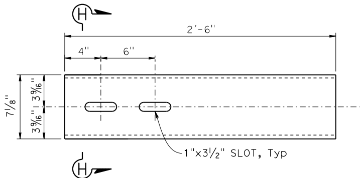
EXPANSION SLEEVE DETAIL (FOR HSS8x4x5/16 RAIL)
