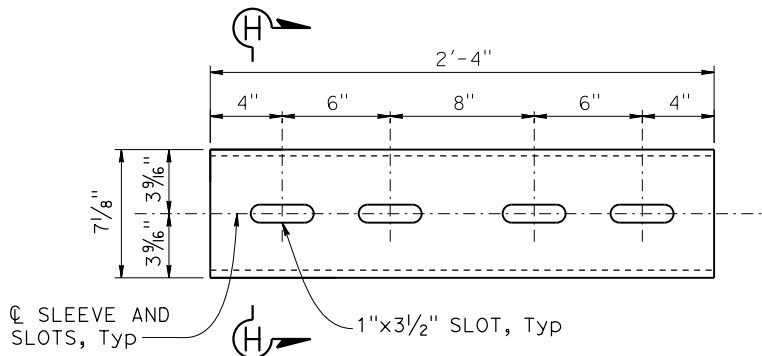
STANDARD SLEEVE DETAIL (FOR HSS8x4x5/16 RAIL)
