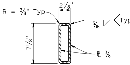
SECTION I-I
