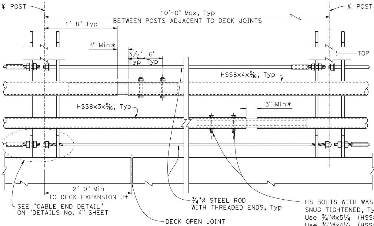
EXPANSION SPLICE *MATCH DECK OR WALL JOINT See Notes 2 and 4
