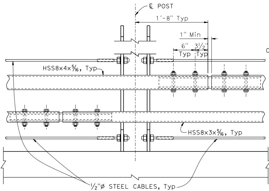
SECTION S-S
