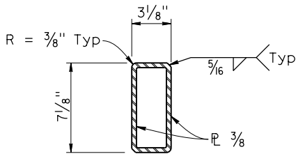
SECTION H-H
