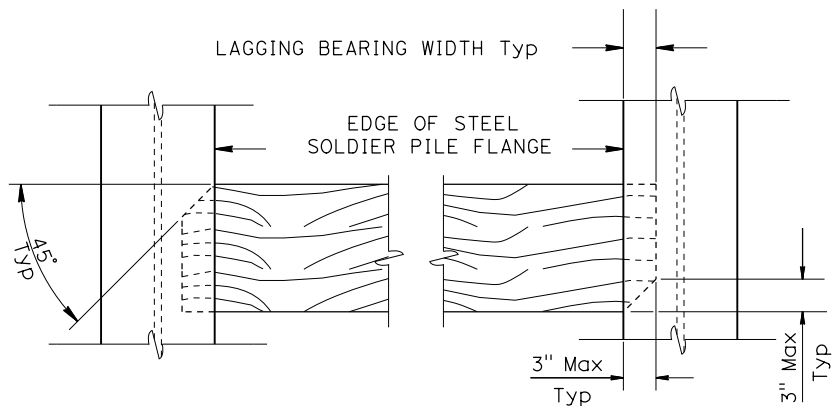
LAGGING CORNERS TRIM DETAIL NO SCALE
