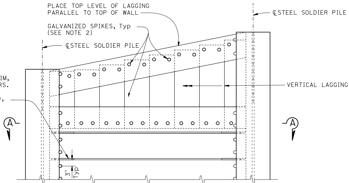
PART ELEVATION LAGGING DETAILS (ALTERNATIVE 2) NO SCALE
