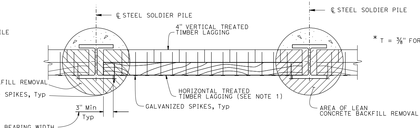
SECTION A-A NO SCALE
