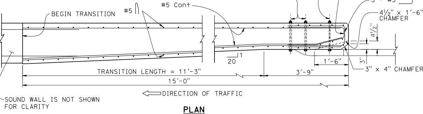
PLAN
