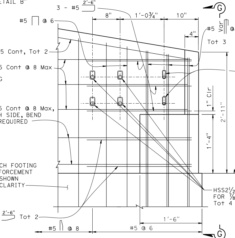
DETAIL B
