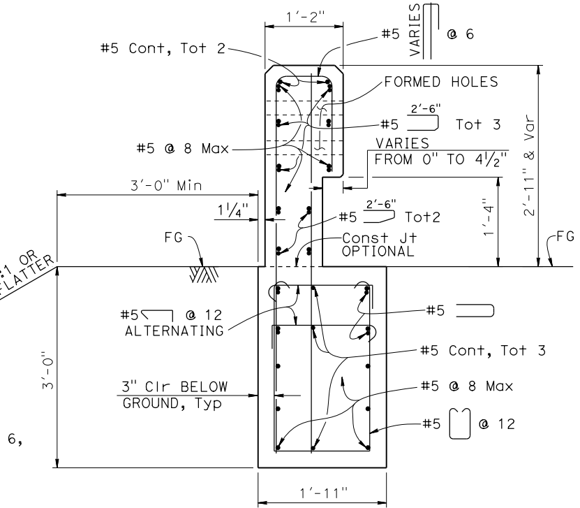
SECTION F-F
