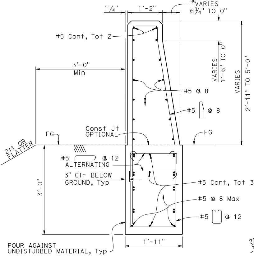
SECTION E-E
