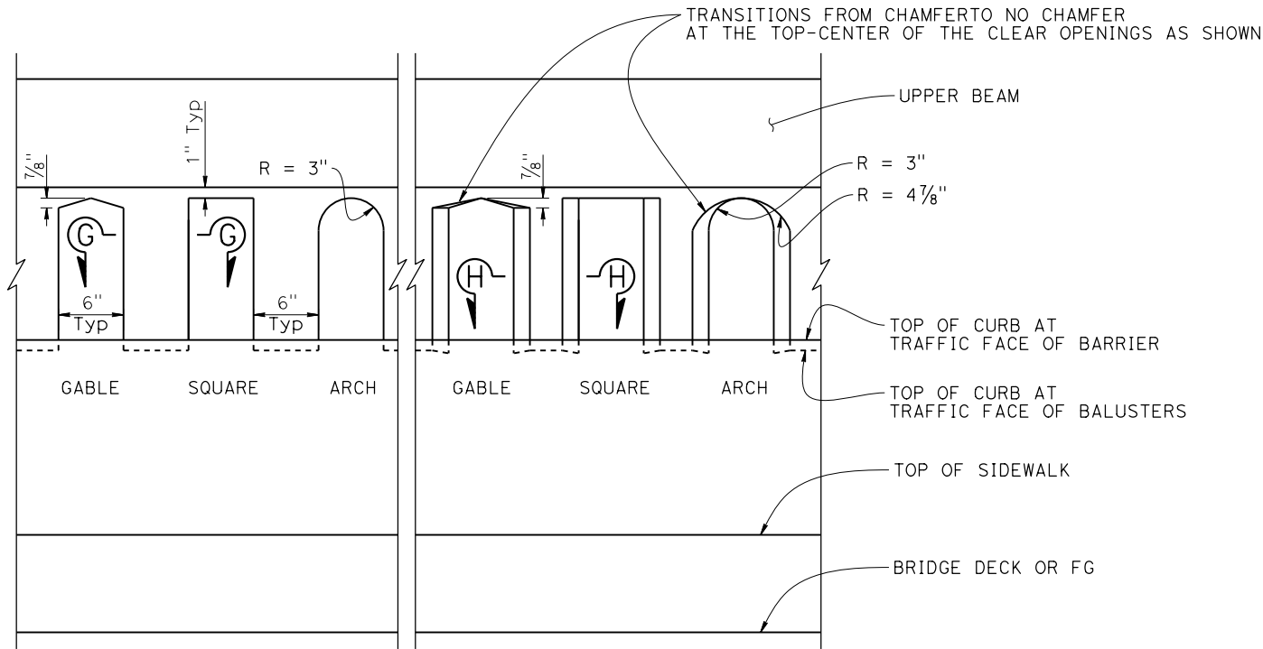
ELEVATION WITH SQUARED BALUSTERS
