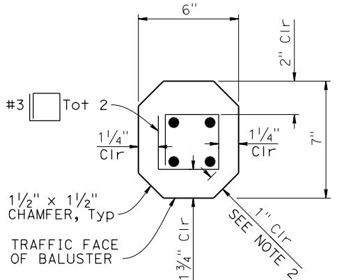
SECTION H-H
