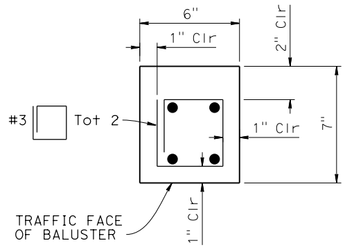
SECTION G-G
