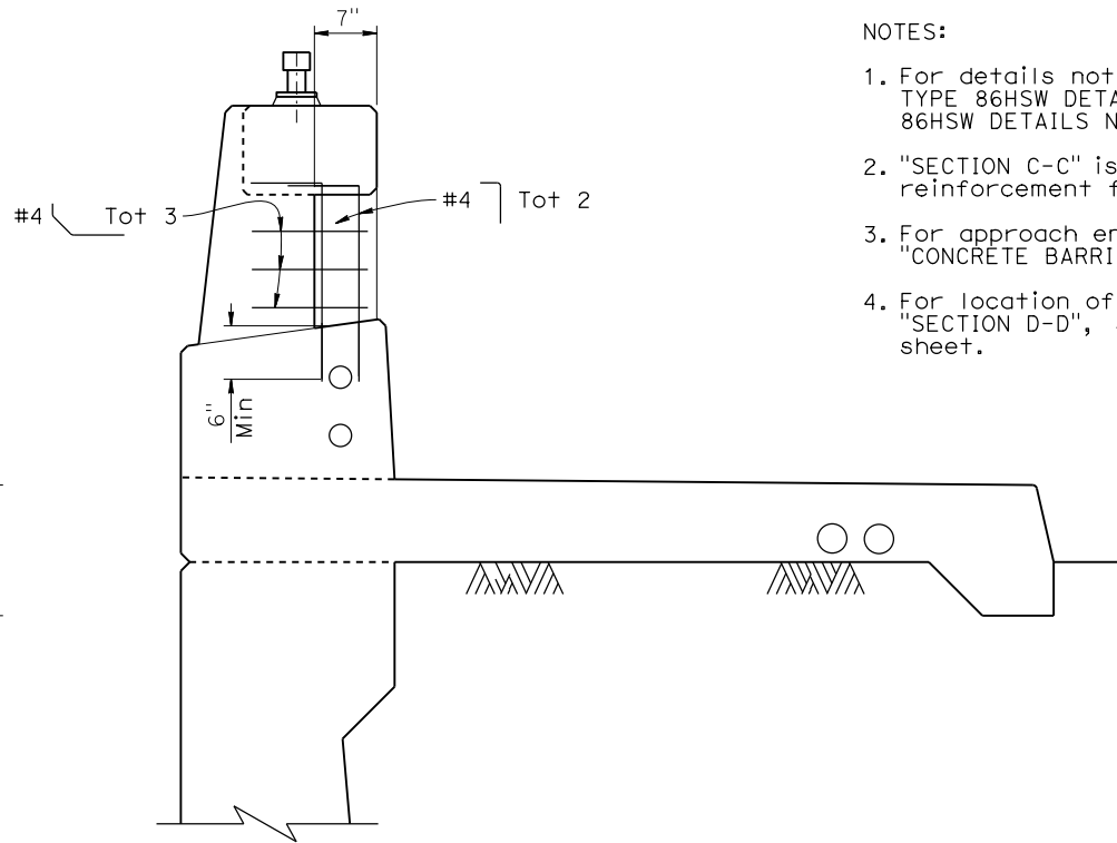
SECTION C-C
