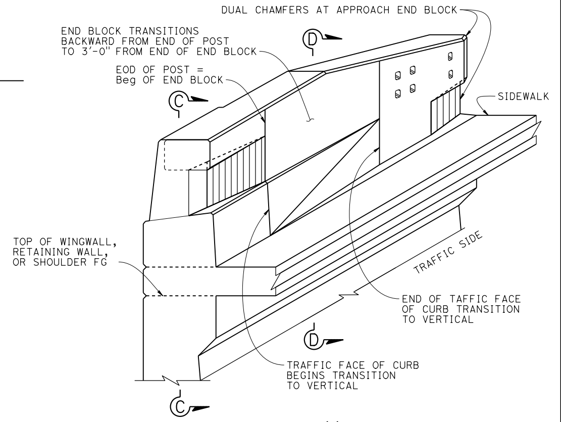
PERSPECTIVE OF POST FACE TRANSITION TO END BLOCK AND DUAL END BLOCK CHAMFERS
