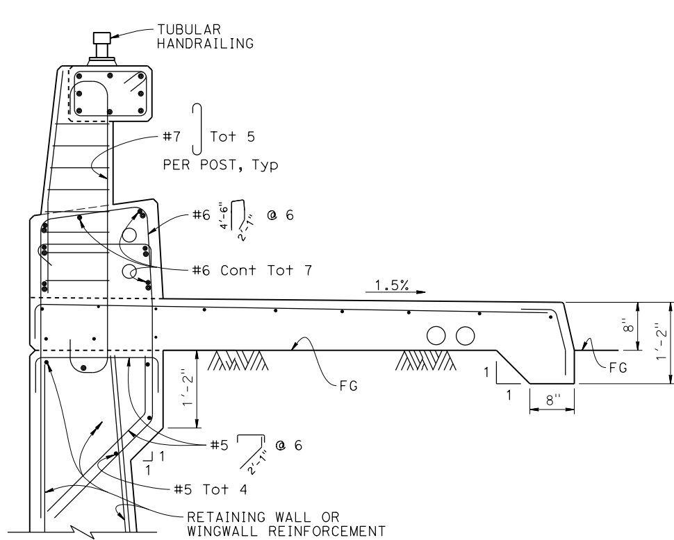
TYPE 86HSA
