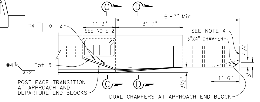
END BLOCK & ADJACENT POST TRANSITION
