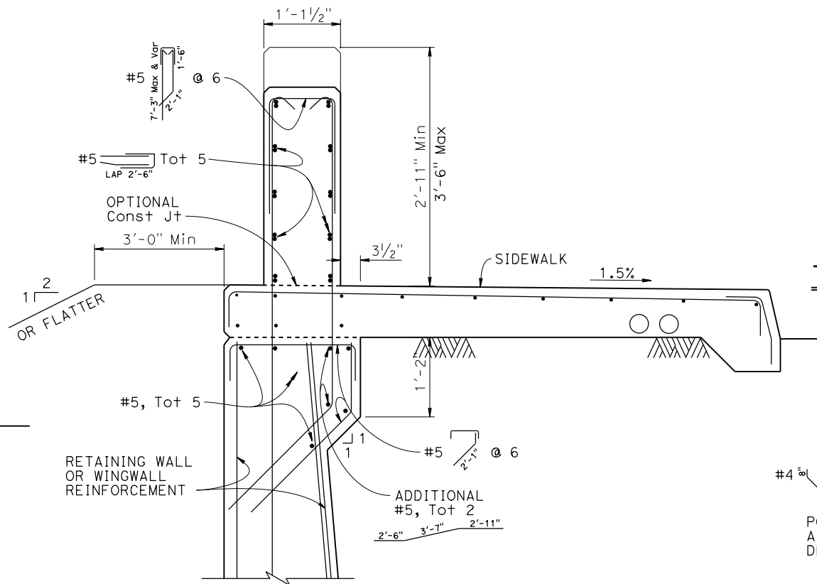
SECTION E-E
