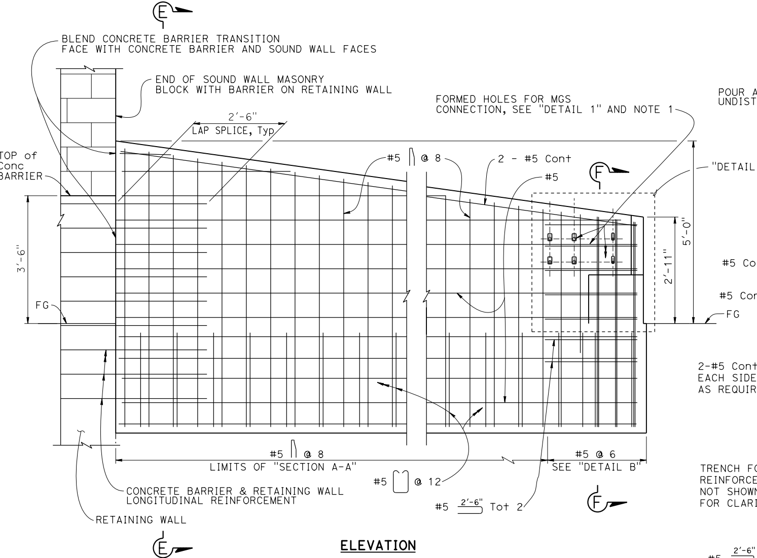
CONCRETE BARRIER TRANSITION AT APPROACH See Note 2
