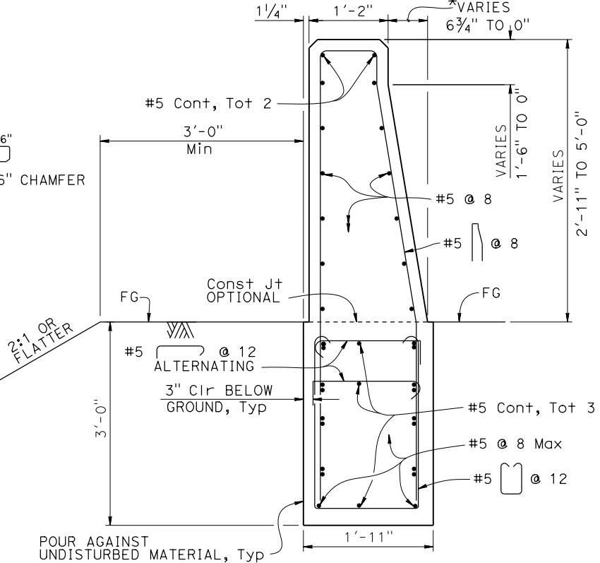
SECTION E-E
