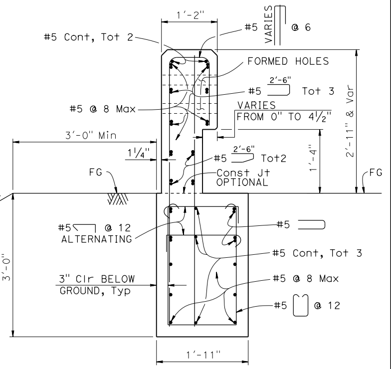
SECTION F-F
