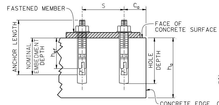
TYPICAL STUD TYPE (WEDGE) STUD MEA
