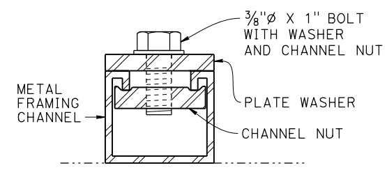
SECTION C-C NO SCALE
