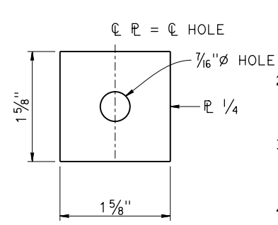
PLATE WASHER NO SCALE
