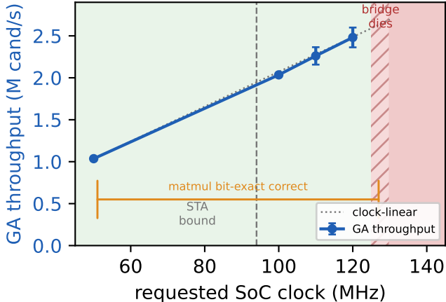
Overclocking a real ECP5-85 past STA
