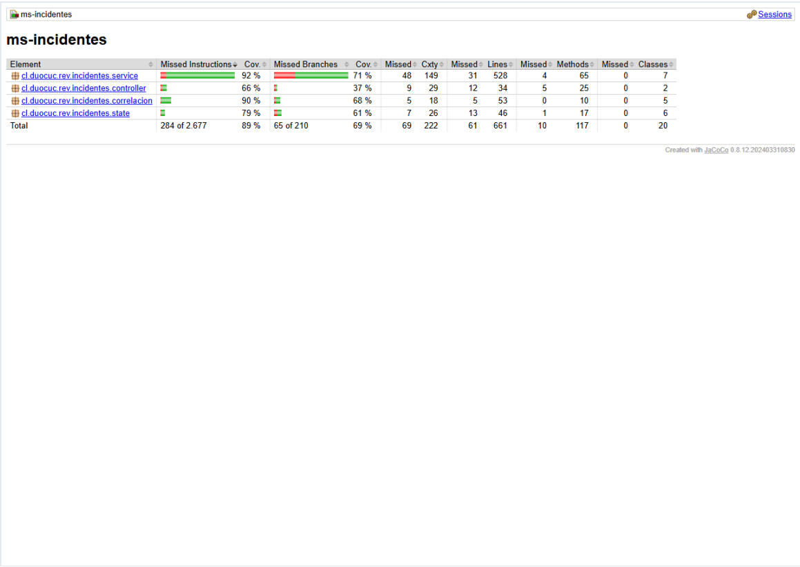
JaCoCo ms-incidentes
