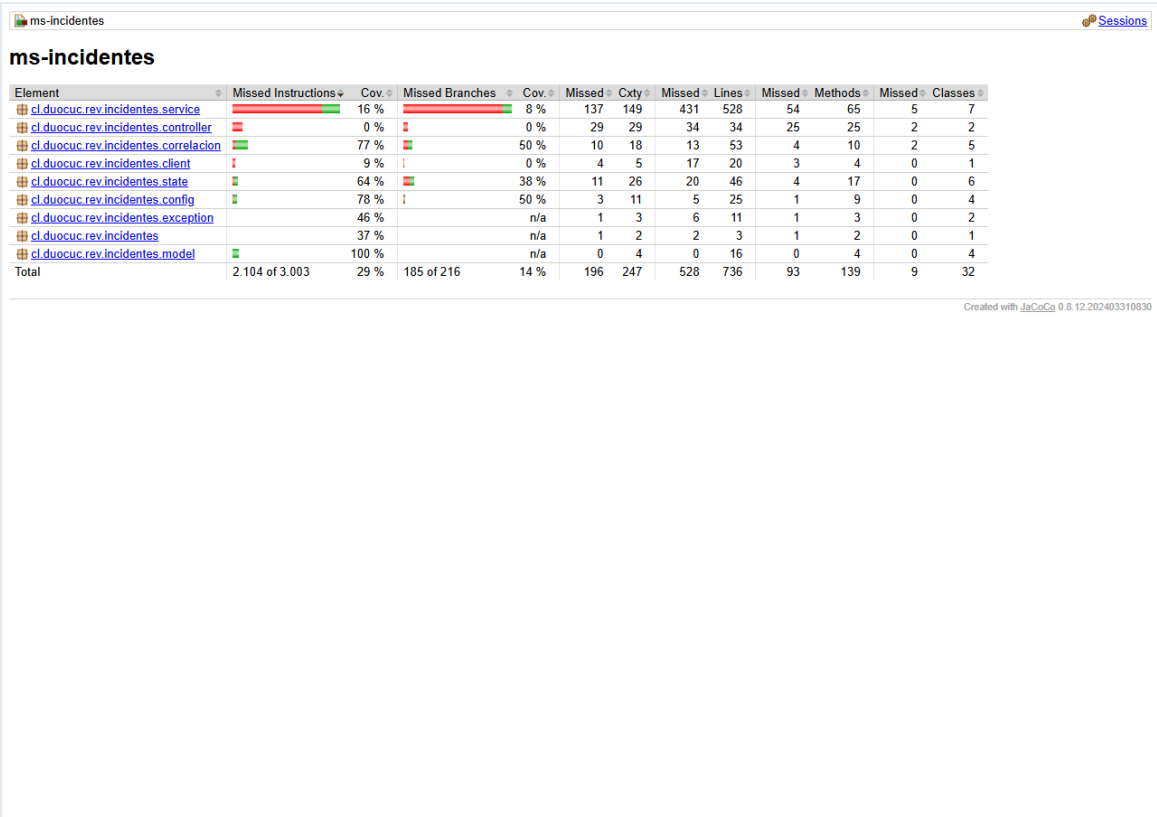
JaCoCo ms-incidentes
