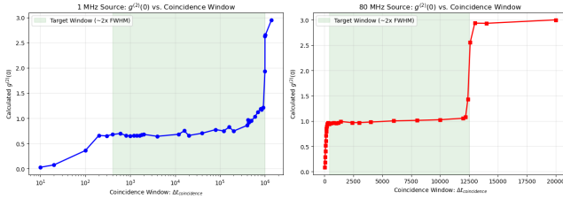
Figure 6: g^2(0) measurement detailed in experiment 0.3.
