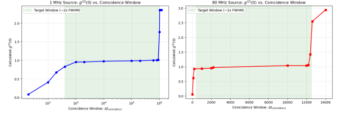
Figure 10: g^{(2)}(0) measurement detailed in experiment 0.3.
