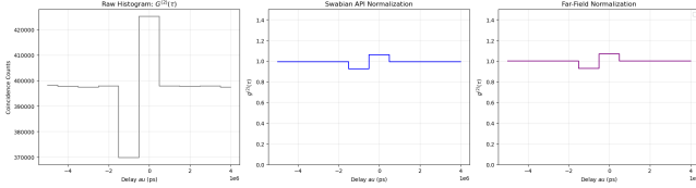
Figure 13: Autocorrelation function measurement.
