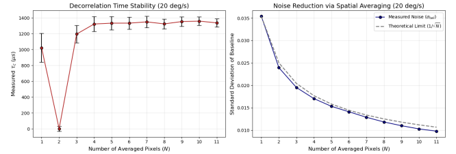
Figure 19: Effect of averaging multiple pixels. The measured \tau_c remains stable (Left), while the noise drops with 1/\sqrt{N} (Right).
