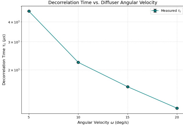
Figure 20: Decorrelation time ( \tau_c ) measured at different diffuser speeds. As angular velocity increases, \tau_c proportionally decreases.
