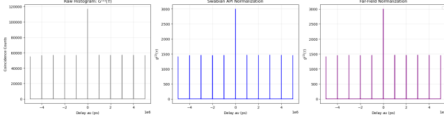
Figure 12: Autocorrelation function measurement.
