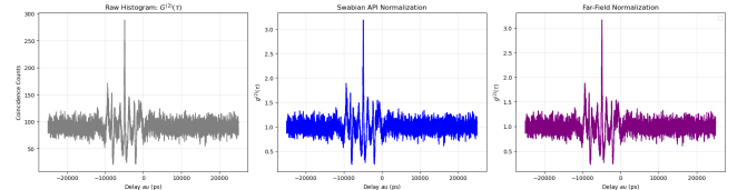
Figure 16: Autocorrelation function measurement for a thermal lamp.
