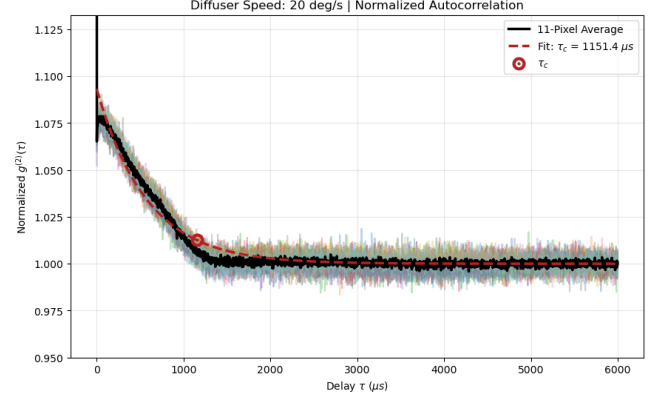
Figure 18: Normalized autocorrelation measurement for the rotating diffuser. The black line is the average of 11 pixels, which is fitted with an exponential curve (red dashed line) to extract \tau_c .
