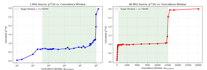
Figure 6: g^{(2)}(0) measurement detailed in experiment 4.1.
