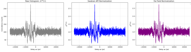
Figure 17: Autocorrelation function measurement for LabLight.
