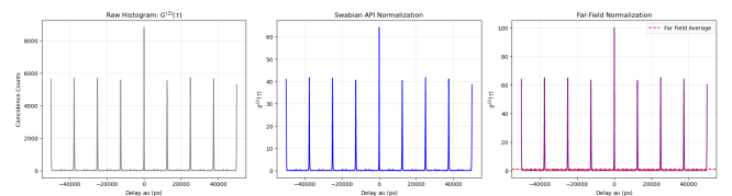
Figure 11: Autocorrelation function measurement for the LASER operating at 80MHz with its respective period of 12,500ps.
