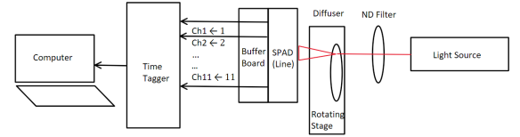
Figure 19: Dynamic speckle setup measurement. CW laser incident onto the rotating diffuser with the SPAD detector array positioned behind it (left).
