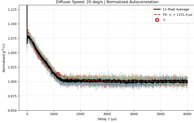
Figure 20: Normalized autocorrelation measurement for the rotating diffuser. The black line is the average of 11 pixels, which is fitted with an exponential curve (red dashed line) to extract \tau_c .
