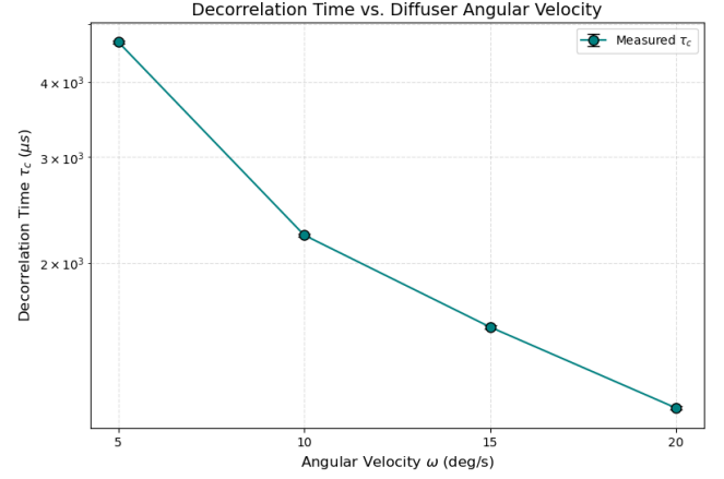
Figure 22: Decorrelation time ( \tau_c ) measured at different diffuser speeds. As angular velocity increases, \tau_c proportionally decreases.
