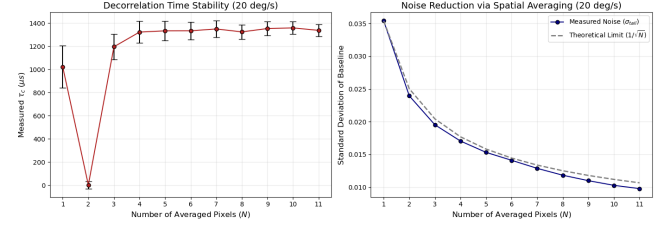
Figure 20: Effect of averaging multiple pixels. The measured \tau_c remains stable (Left), while the noise drops with 1/\sqrt{N} (Right).
