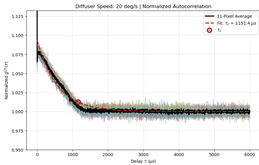
Figure 19: Normalized autocorrelation measurement for the rotating diffuser. The black line is the average of 11 pixels, which is fitted with an exponential curve (red dashed line) to extract \tau_c .
