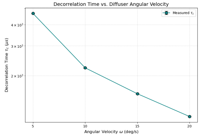
Figure 21: Decorrelation time ( \tau_c ) measured at different diffuser speeds. As angular velocity increases, \tau_c proportionally decreases.
