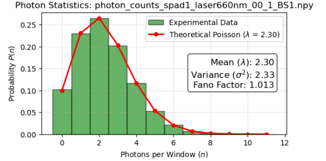
Figure 4: Photon count distribution (0.1mW).
