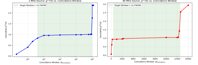
Figure 9: g^{(2)}(0) measurement detailed in experiment 0.5.
