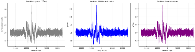
Figure 17: Cross-correlation function measurement for the laboratory light.
