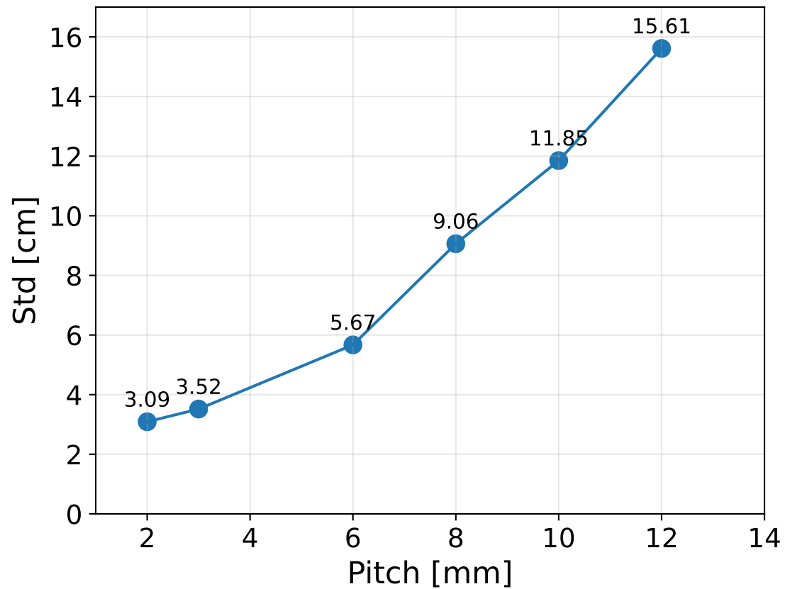
Std of ( z_{\text{rec}} - z_{\text{true}} )
