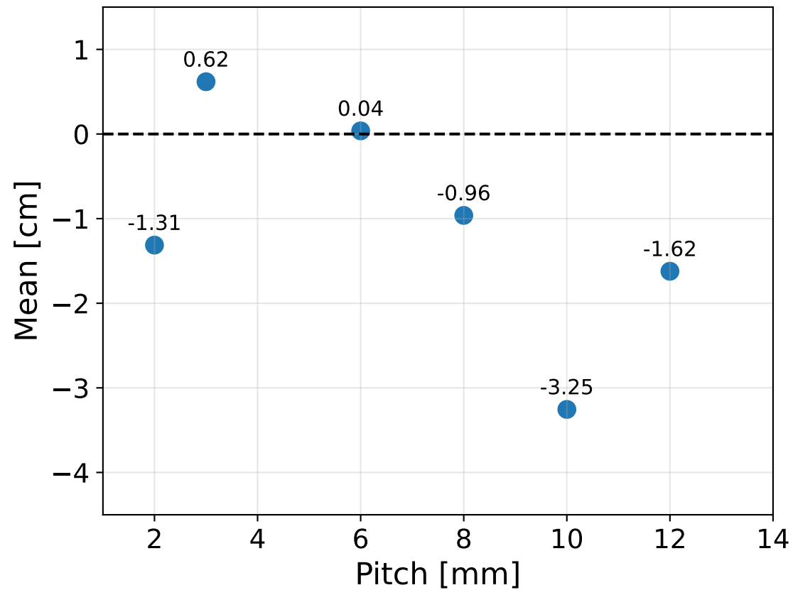
Mean of ( z_{\text{rec}} - z_{\text{true}} )
