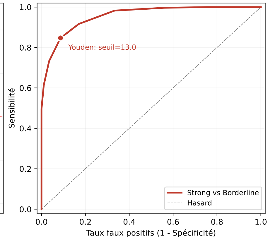
(c) Discrimination strong vs borderline AUC = 0.956 [IC95 : 0.953, 0.958]
