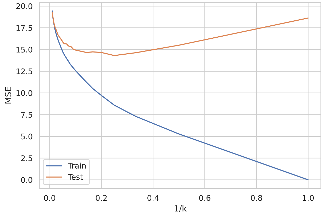
KNN: Normalized Features
