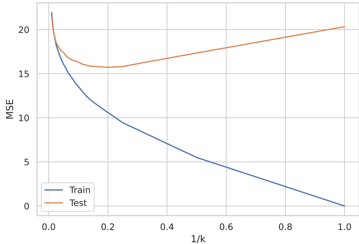
KNN: Raw Features
