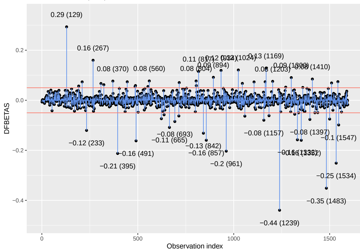
DFBETAS values for coefficient of PctPopUnderPov.PctBSorMore Thresholds are at \pm(2\div vn)
