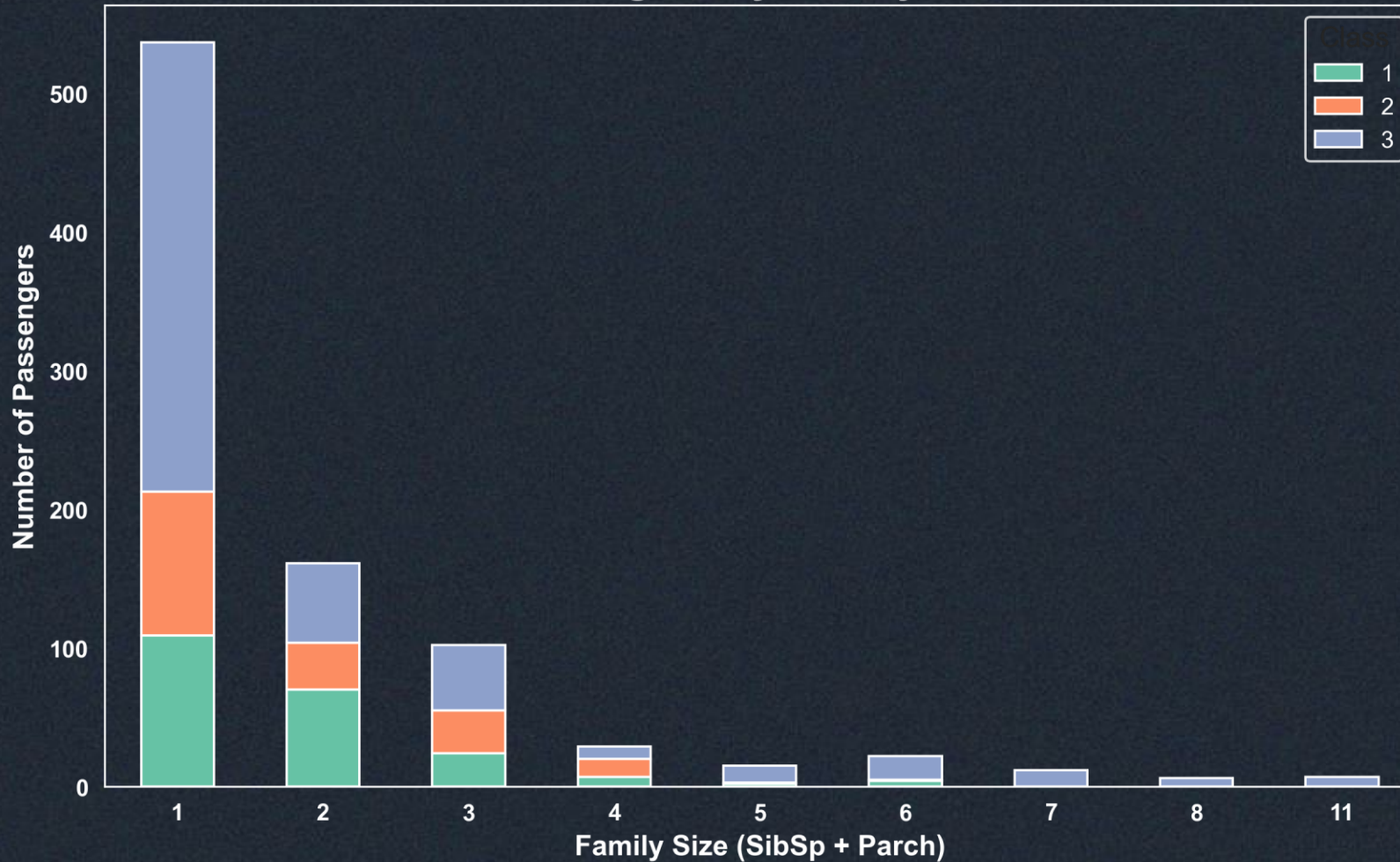
Count of Passengers by Family Size and Class
